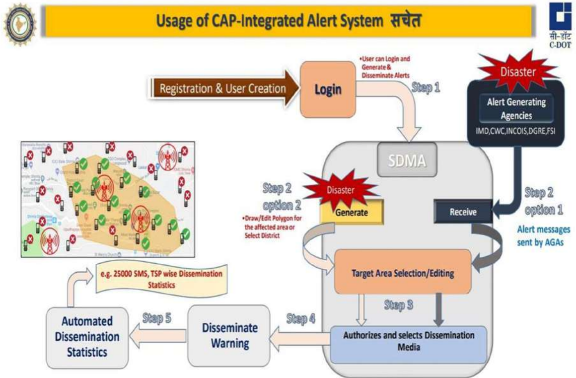
Flow Process of Sachet
