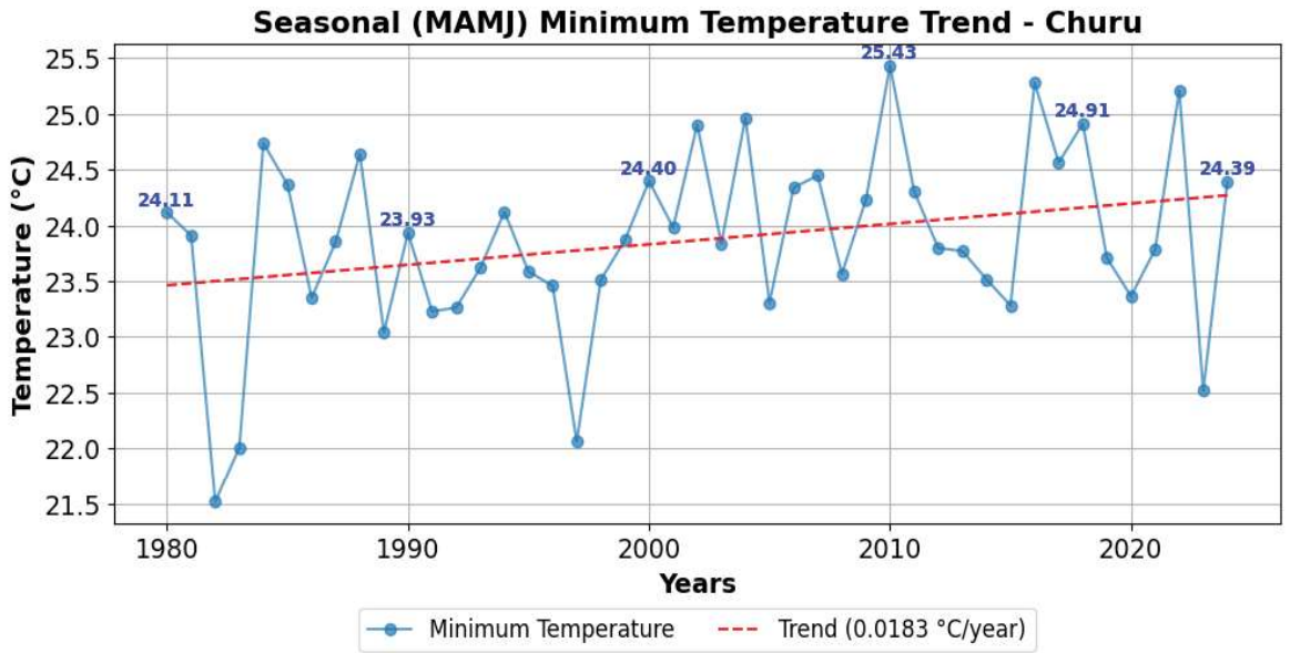
Figure 4: Seasonal – March to June (MAMJ) Minimum Temperatures in Churu from 1980-2024 (Source: NRDC India)
